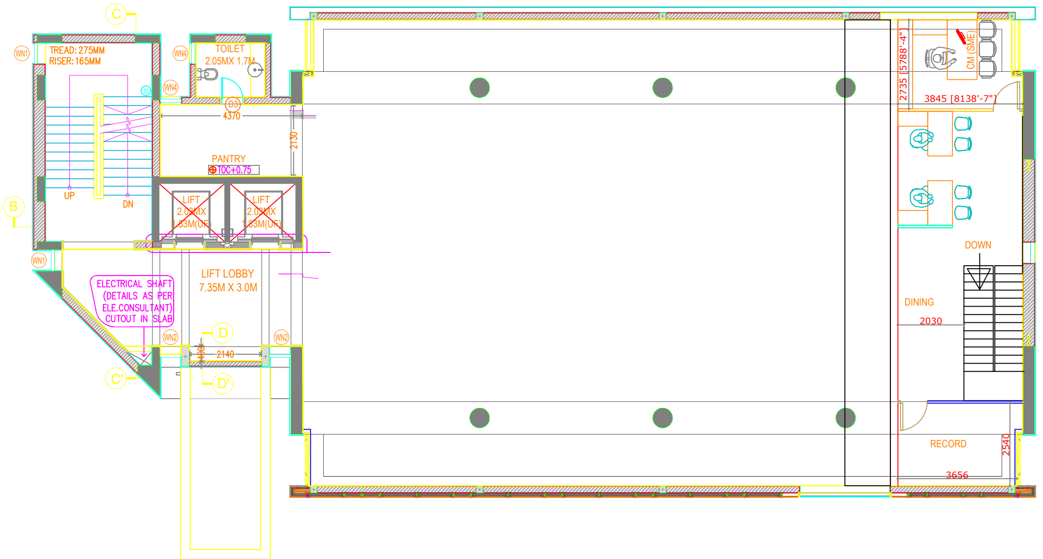
LAYOUT FOR NIGDI BRANCH - PUNE WEST FIRST FLOOR
