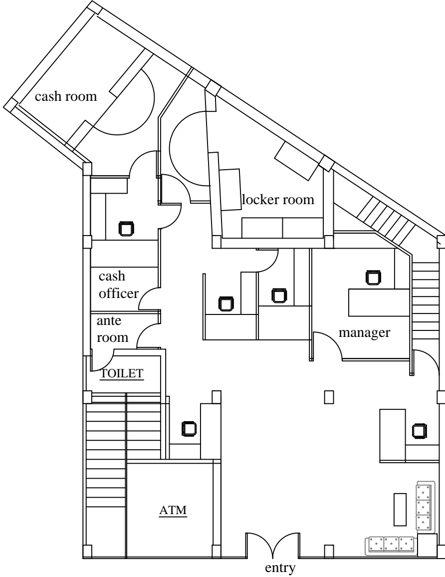
SBI NERIAMANGALAM BRANCH LAYOUT PLAN (GF)
