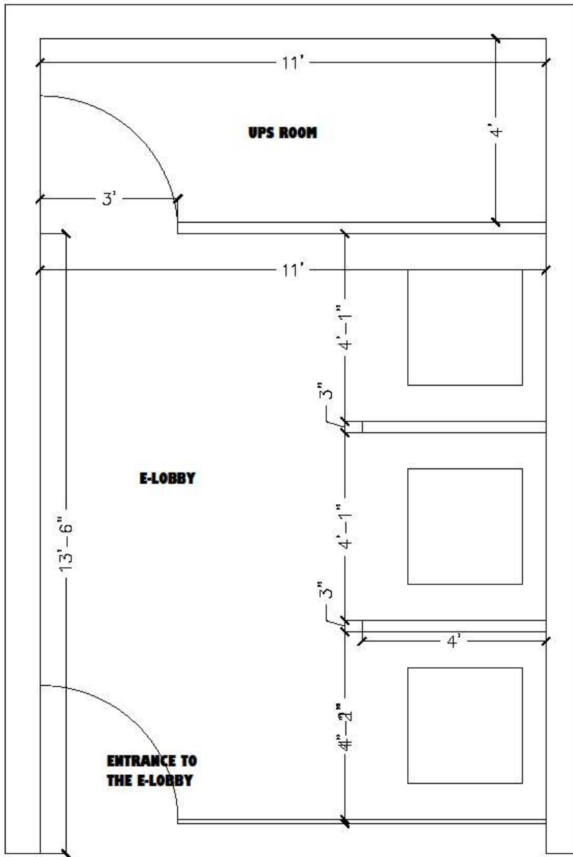
PLAN OF TCA E-LOBBY
