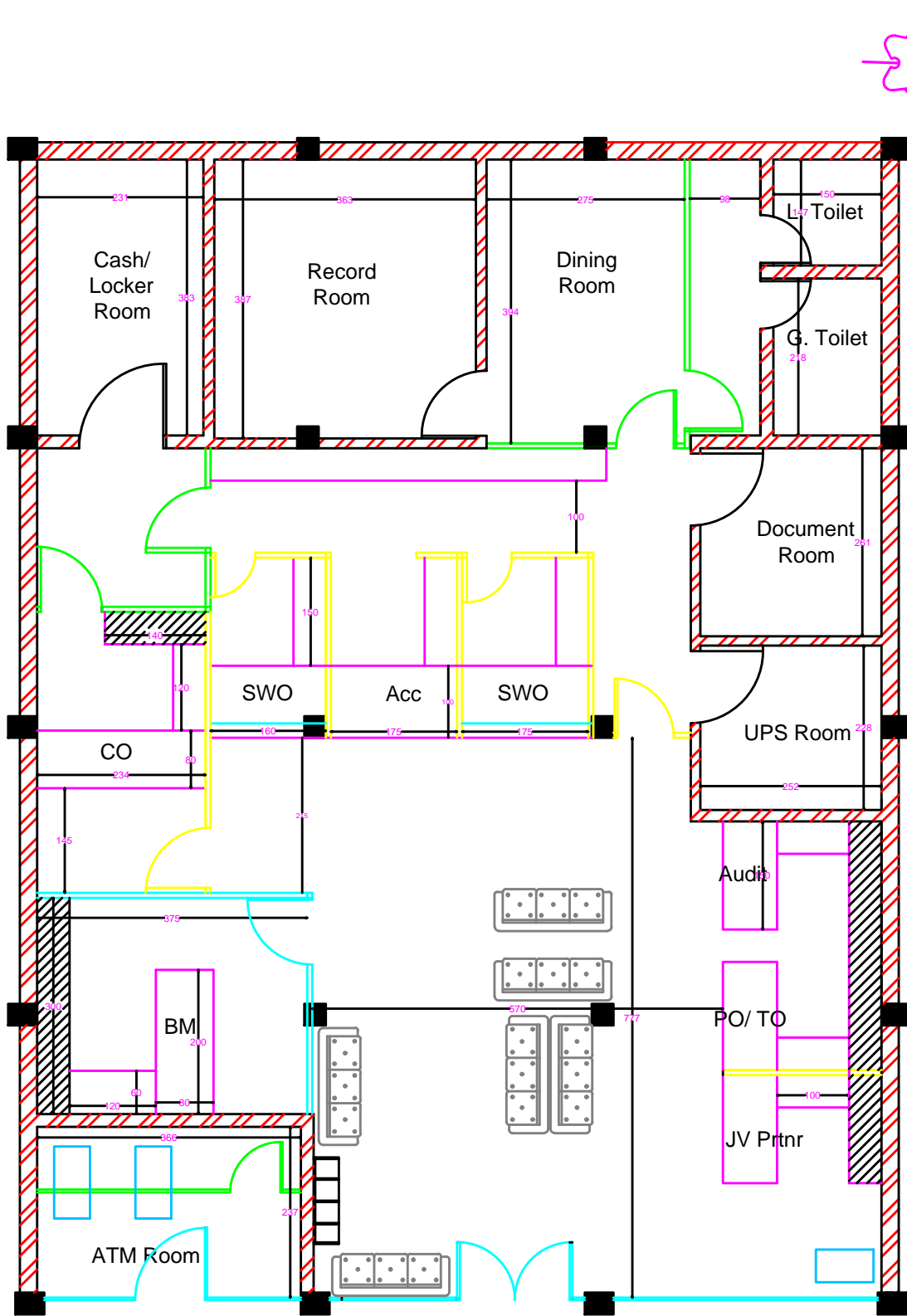
SBI KAVARATTI BRANCH - PROPOSED LAYOUT PLAN (Option 1 - without extension)
