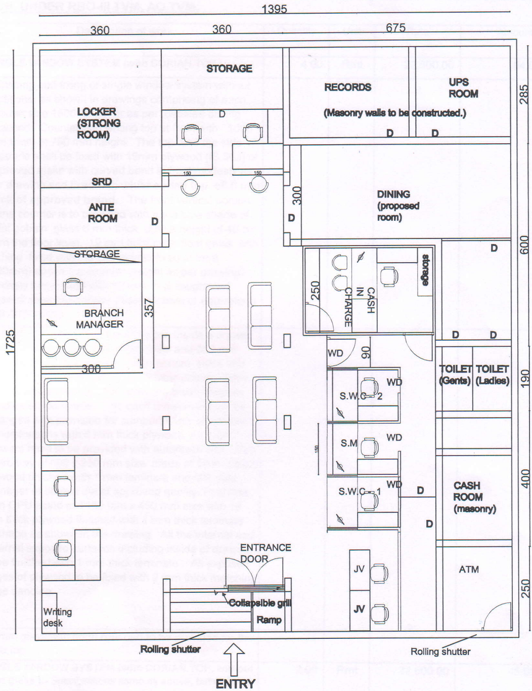
SBI SREEKARYAM BRANCH PROPOSED RENOVATION LAYOUT - Dwg -01 dated 22.03.2023
