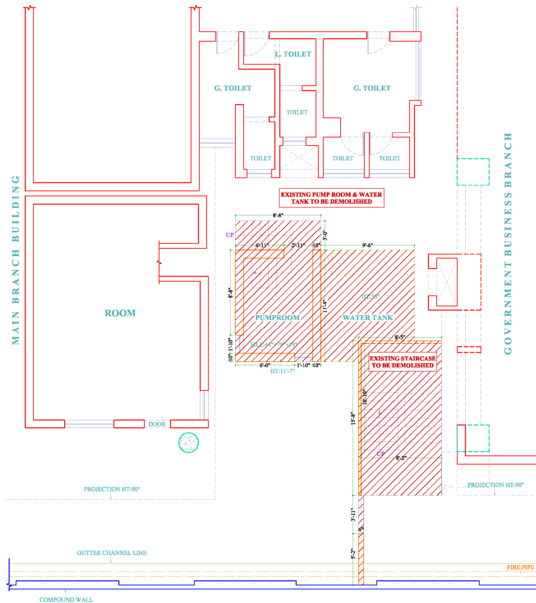
DEMOLITION DRAWING FOR WATERTANK AT SBI MANDVI BRANCH, VADODARA.
