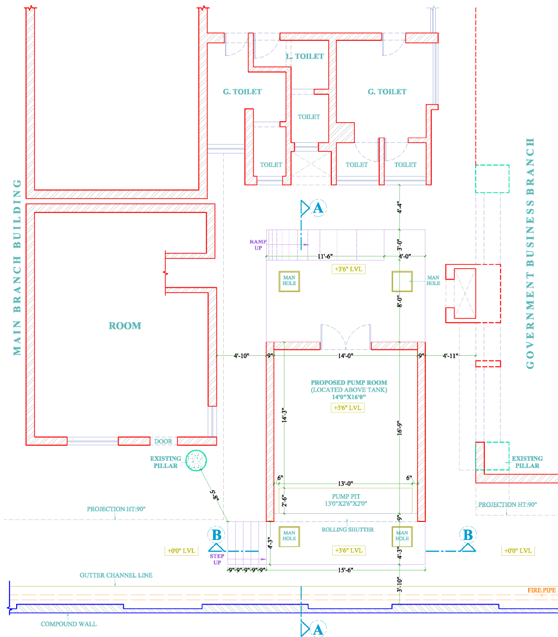
CIVIL LAYOUT PLAN OF PUMP ROOM AT SBI MANDVI BRANCH, VADODARA.
