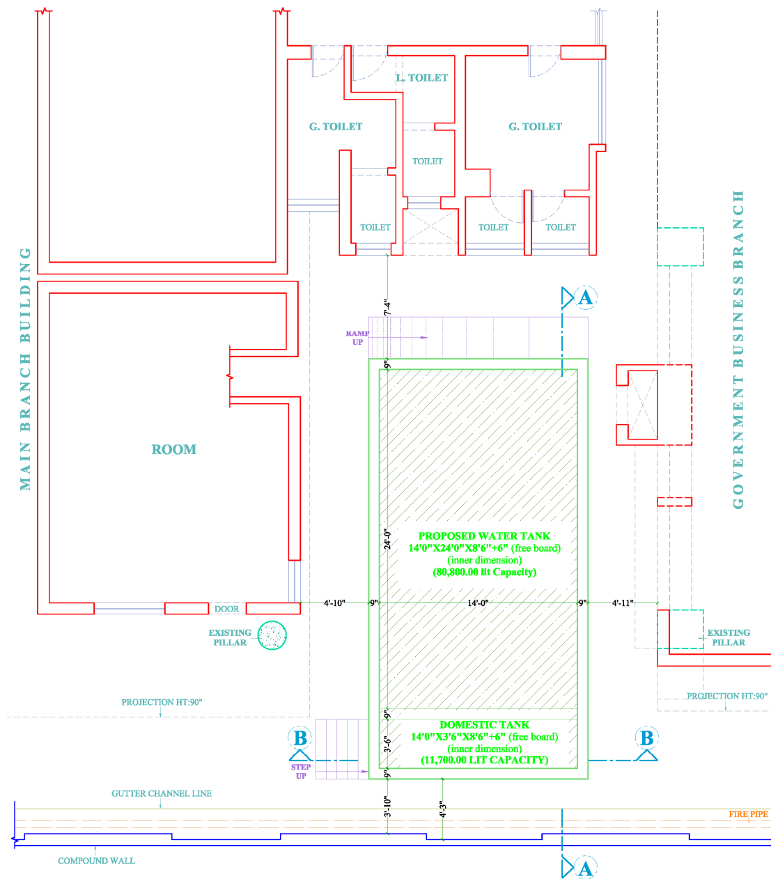
CIVIL LAYOUT PLAN OF WATERTANK AT SBI MANDVI BRANCH, VADODARA.
