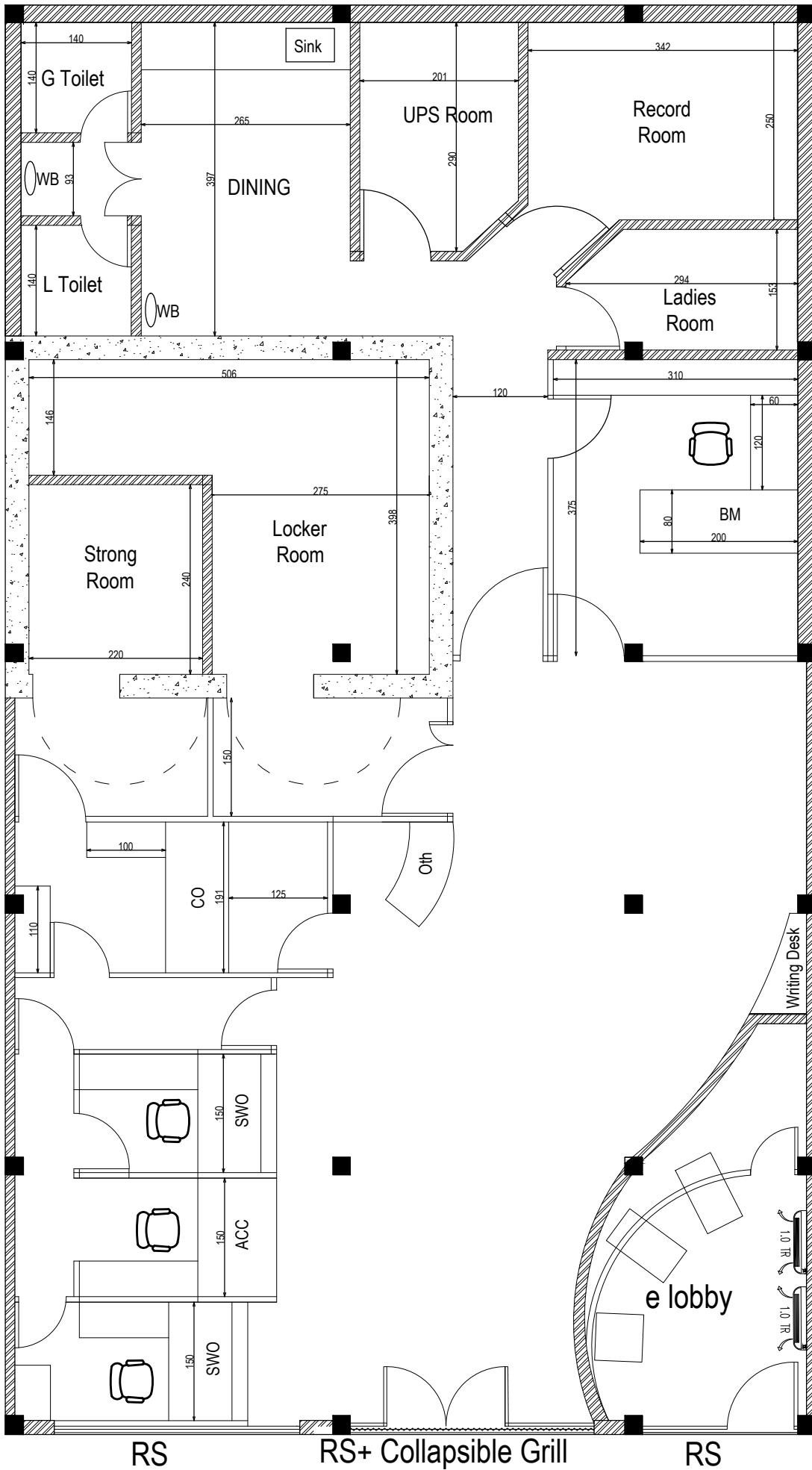
LAYOUT PLAN OF SBI ANDROTH BRANCH
