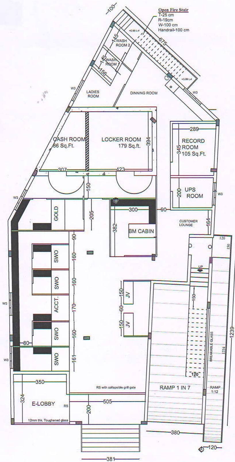
PROPOSED LAYOUT FOR AZHIKODE BRANCH APPROX .B.U.P AREA 2743 =Sq .Ft.
