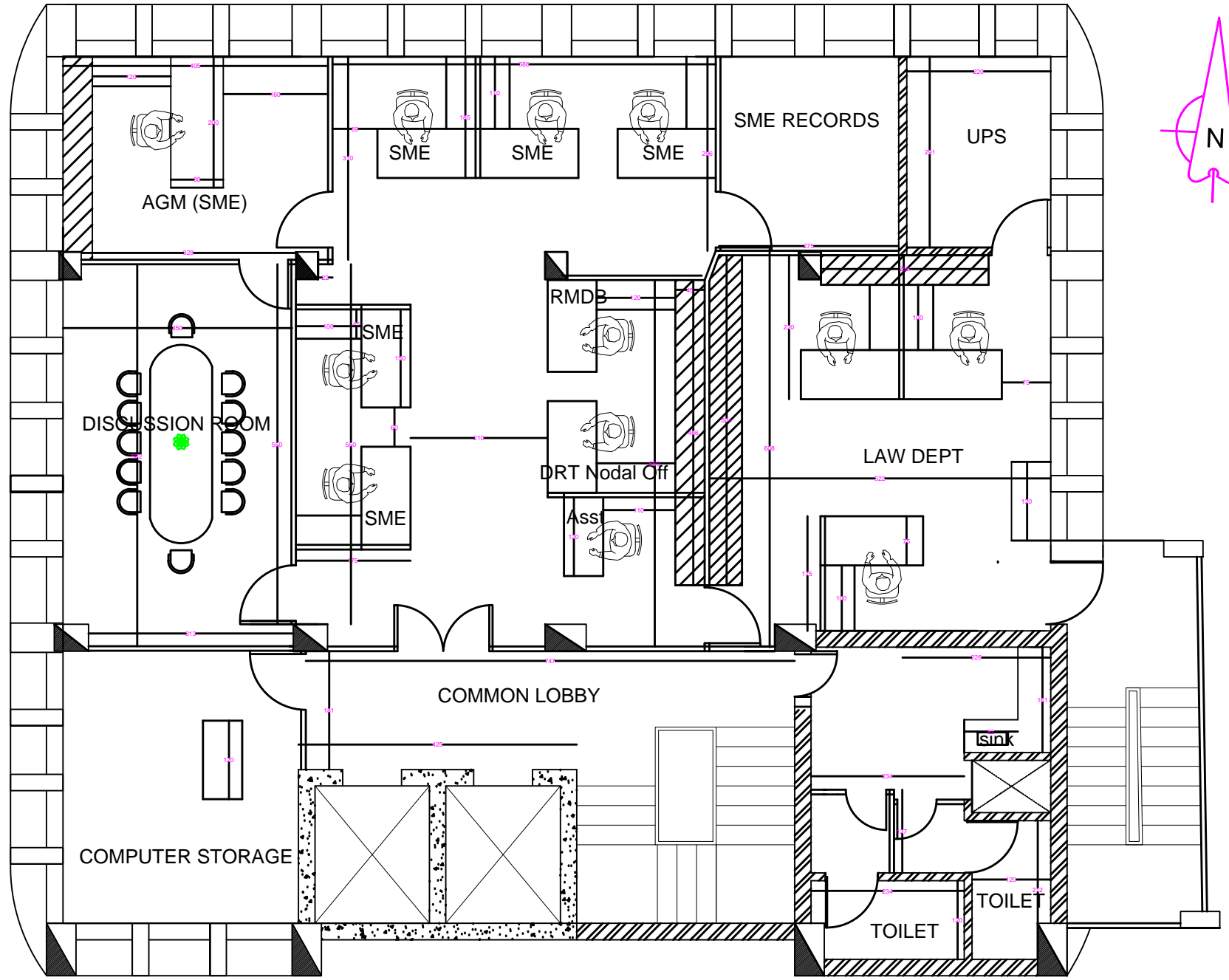
PROPOSED LAYOUT OF 7TH FLOOR
