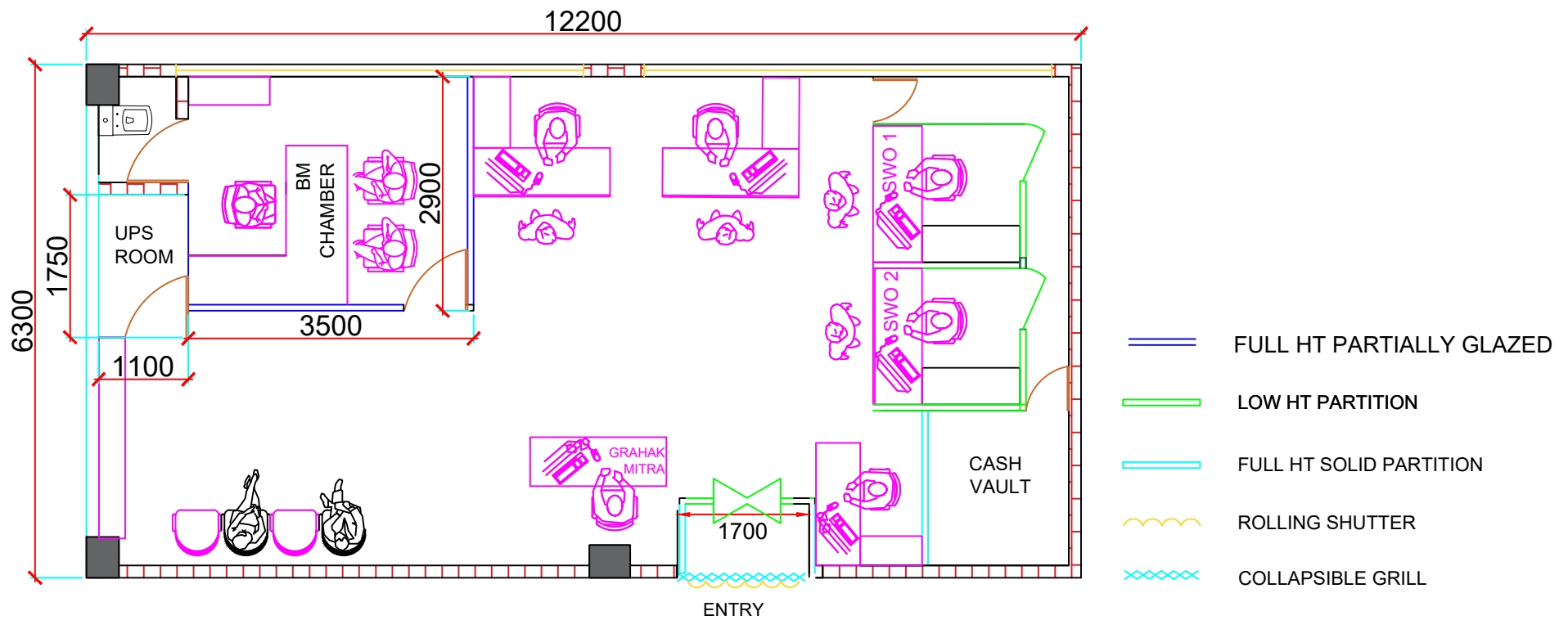
FIG : PROPOSED LAYOUT OF NEW SECRETARIAT, AGARTALA BRANCH
