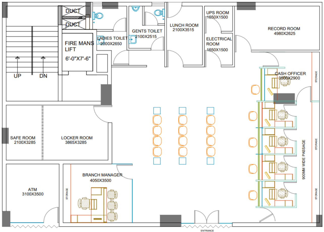
DRAWING- PROPOSED INTERIOR WORKS FOR BEGUMPET BRACH (10676) UNDER RBO SECUNDERABAD, AO SECUNDERABAD
