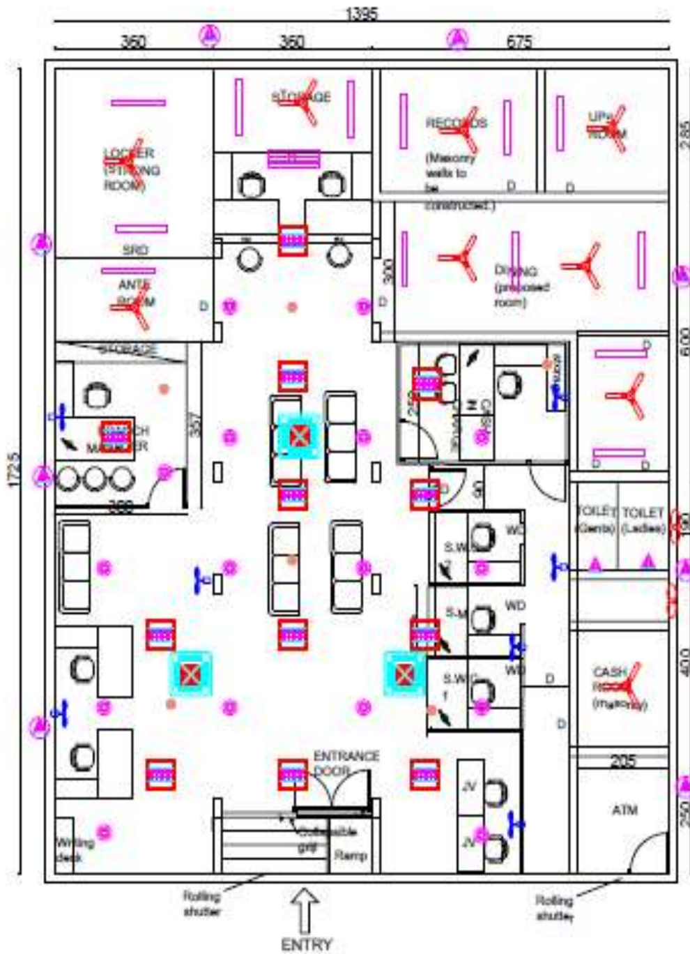
SBI SREEKARYAM BRANCH PROPOSED RENOVATION LAYOUT -
