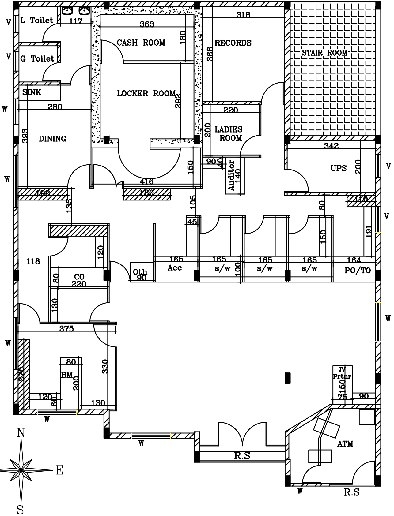
PROPOSED LAYOUT OF SBI MANNAM BRANCH
