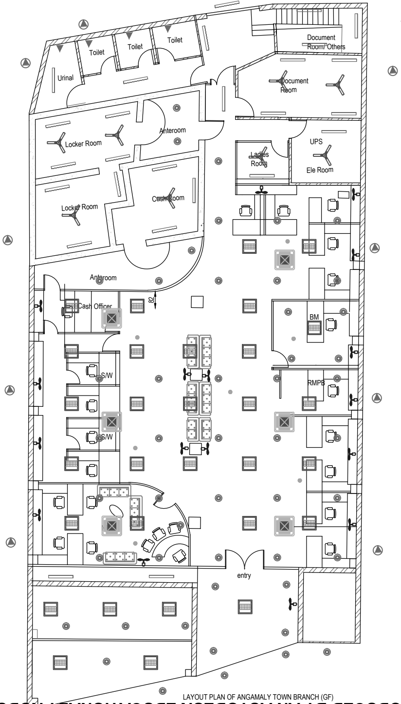
LAYOUT PLAN OF ANGAMALY TOWN BRANCH (GF)
