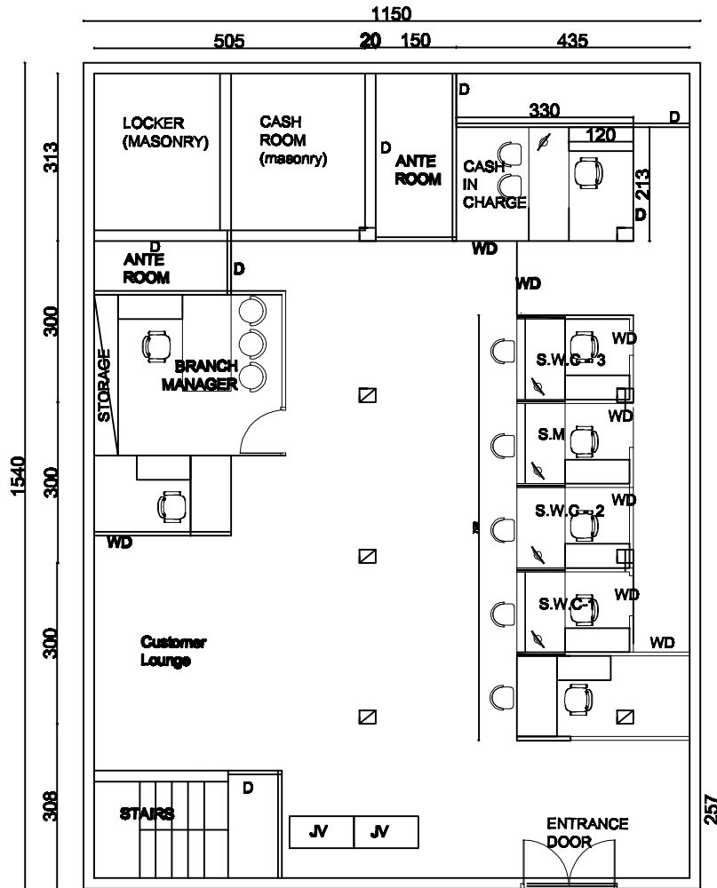
SBI VALIYAVILA BRANCH PROPOSED RENOVATION LAYOUT - Dwg -02 dated 29.05.2023
